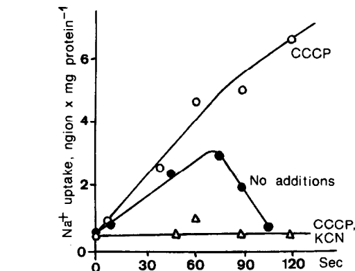
Fig.3. CCCP-stimulated Na + uptake by E. coli inside-out subcellular vesicles oxidizing NADH. Incubation mixture, 50 mM K 2 SO 4 , 5 mM Na 2 SO 4 , 30 mM MgSO 4 , 25 mM potassium acetate, 0.1 M Tricine-KOH (pH 7.75). At zero time, 5 mM NADH was added. Other additions: 1 \times 10^{-5} M CCCP, 10 mM KCN.
